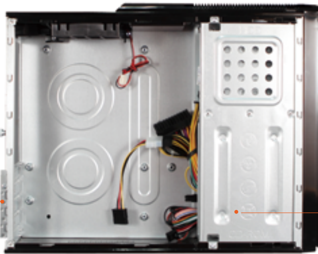
PSU Position
