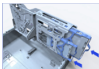
Reverse drive bracket
